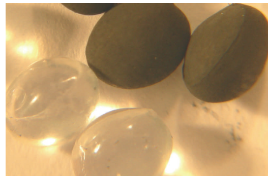
Starting Materials
